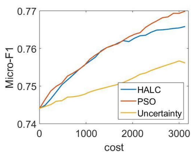
Scop-go
