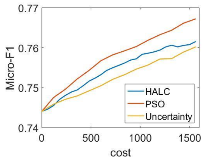
Scop-go
