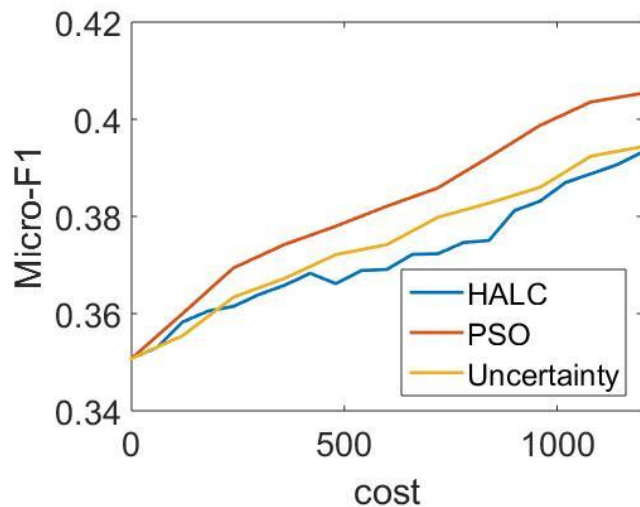
Yeast-go
